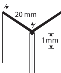
20 x 20 mm Tapettikulmalista | Tapetvinkellist | Corner trim for wallpaper
